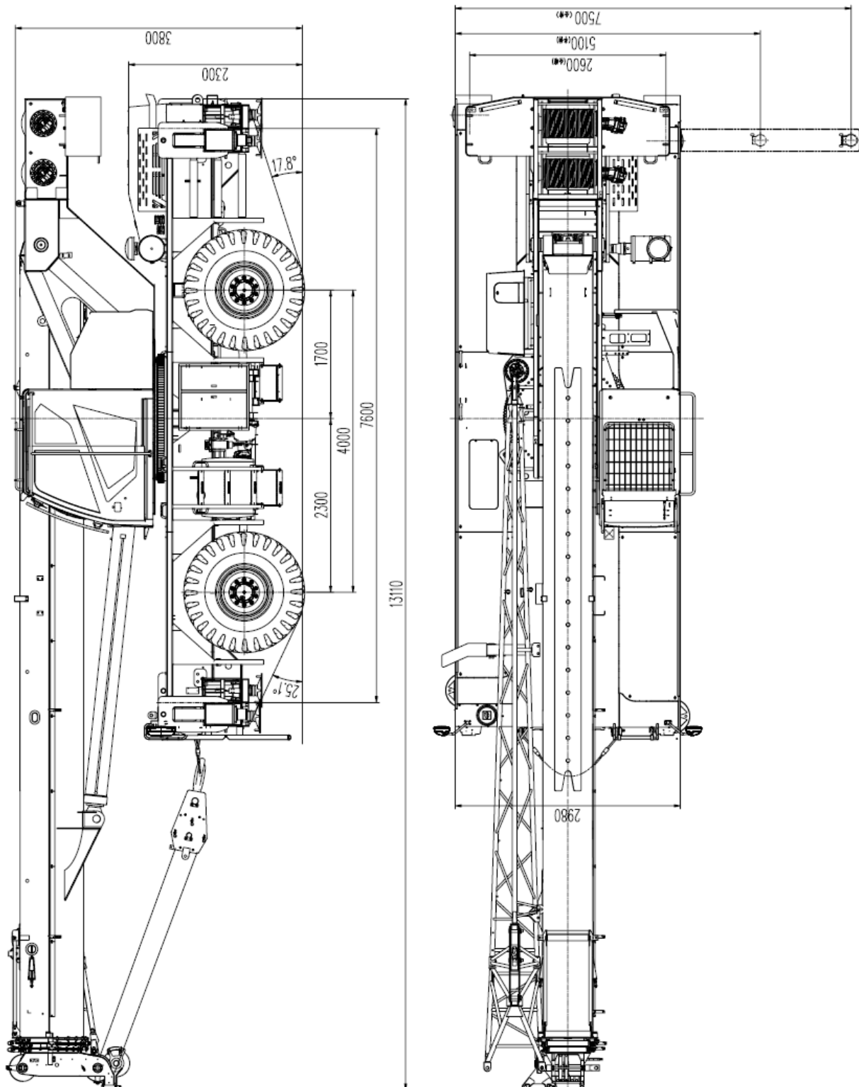
Figure 1 Overall View – ZRT500V432 Rough Terrain Crane
